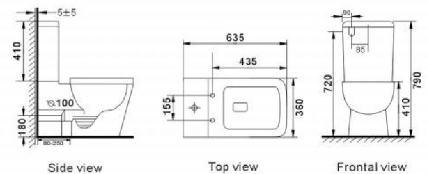
B2040A Washdown two piece toilet Size: 635x360x790 mm
